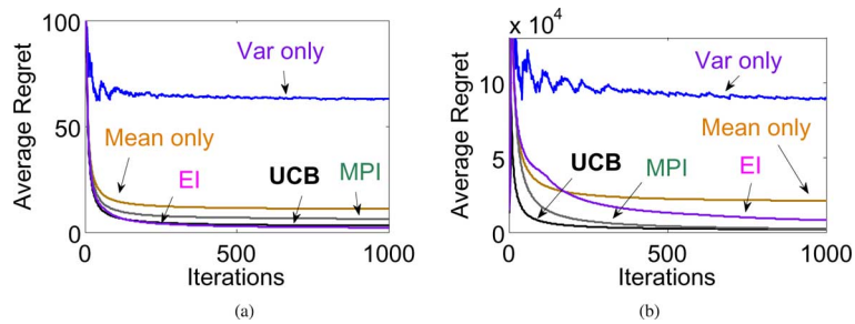
Fig. 10. Comparison of GP-UCB and various heuristics on (a) Branin and (b) Goldstein-Price benchmark functions.
