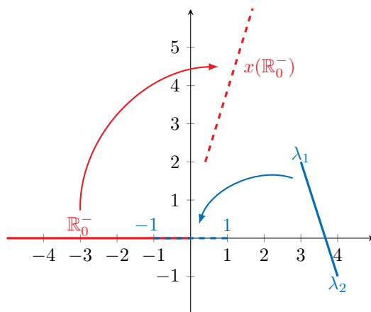
Figure 6. Transformation of the line segment [\lambda_1, \lambda_2] = [3 + 2i, 4 - i] to the interval [-1, 1] and corresponding transformation of the negative real axis.
