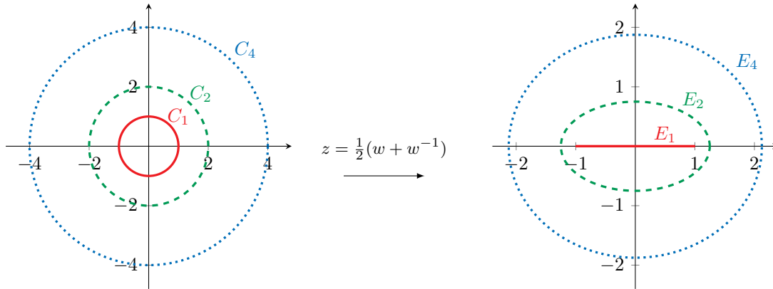
Figure 1. The Joukowski mapping z = \frac{1}{2}(w + w^{-1}) .
