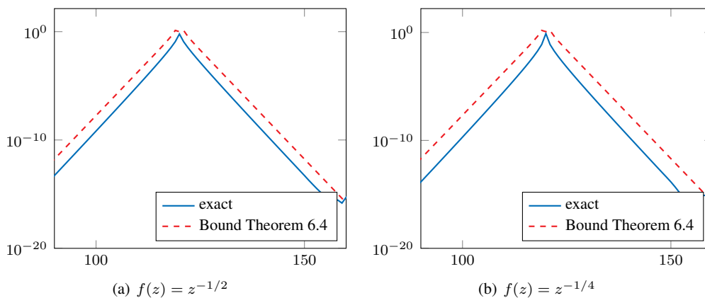
Figure 9. Bounds for [A^{-1/2}]_{k\ell} (left) and [A^{-1/4}]_{k\ell} (right), \ell = 120 for the matrix A = \text{tridiag}(1, i, -1) + 2 \cdot I .
