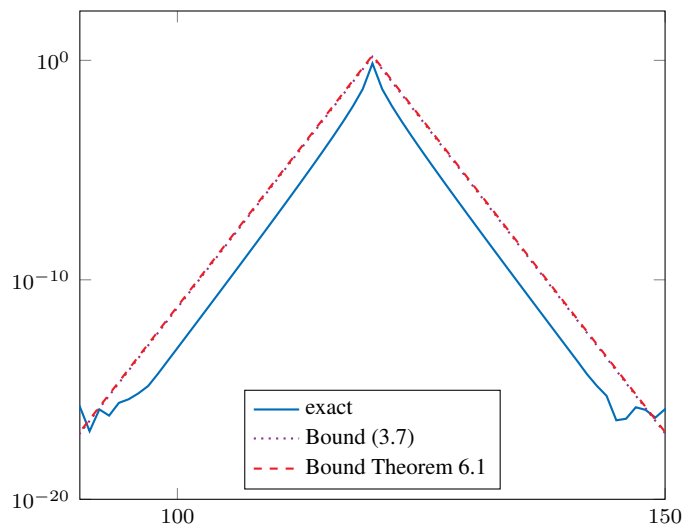
Figure 8. Bounds for [A^{-1/4}]_{k\ell} , \ell = 120 for the matrix A = \text{tridiag}(-1, 4, -1) .
