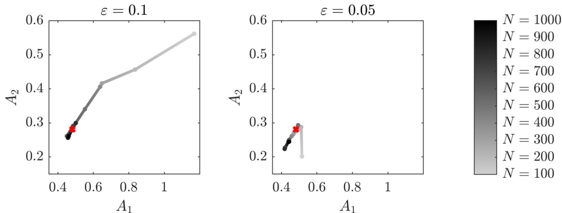
Fig. 6 Evolution in time of the estimator \widehat{A}_{N,J}^\epsilon with J = 1 for a two-dimensional drift coefficient
