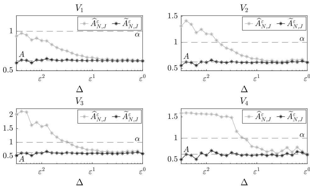
Fig. 5 Comparison between our two estimators \widehat{A}_{N,J}^\epsilon without filtered data and \widetilde{A}_{N,J}^\epsilon with filtered data with J = 1 as a function of the distance \Delta between two successive observations for different slow-scale potentials
