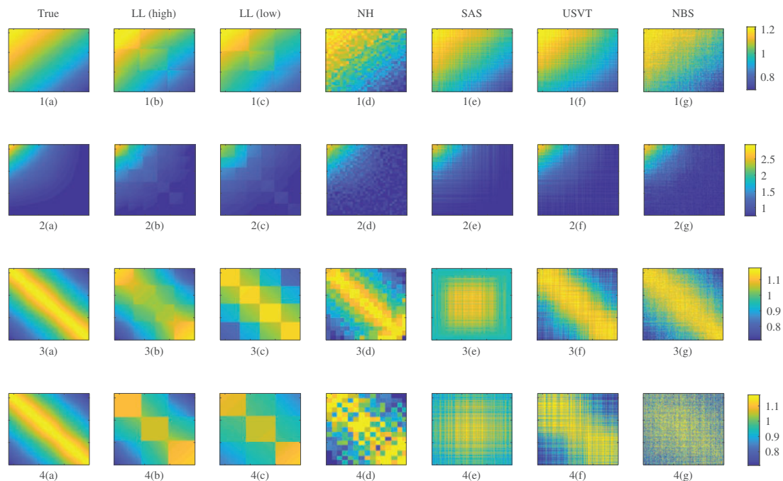
Fig. 1. Graphon estimates from networks of size n = 1600 , with f_1 and \rho_n \propto 1 in the first row, f_2 and \rho_n \propto 1 in the second row, f_3 and \rho_n \propto 1 in the third row, and f_3 and \rho_n \propto n^{-1} \log^3(n) in the fourth row, using the proposed local linear method (LL) under high and low signal-to-noise ratio settings in (b) and (c) and using the network histogram (NH), sort-and-smooth method (SAS), universal singular-value thresholding (USVT) and neighbourhood smoothing (NBS) in (d)–(g).
