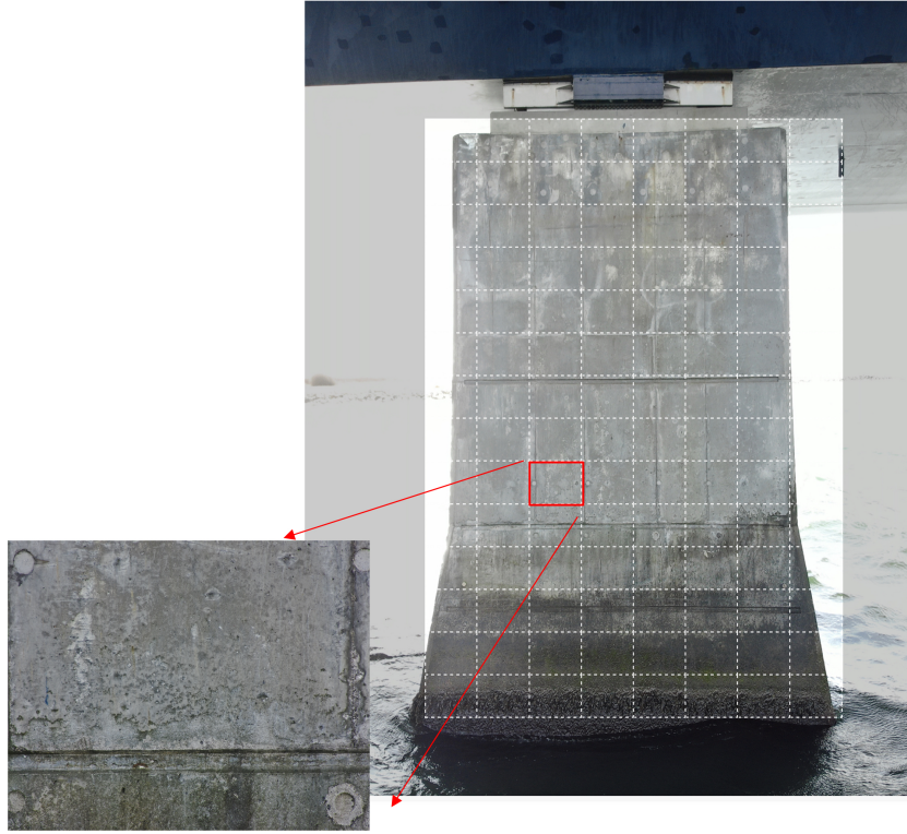
Fig. 2: DJI Matrix 300 Hi-Res Grid: example of a 7-grid of 98 high-resolution images. Each individual image is 5184 \times 3888 pixel in size resulting in a overall data size for a single pillar face of almost 1GB.
