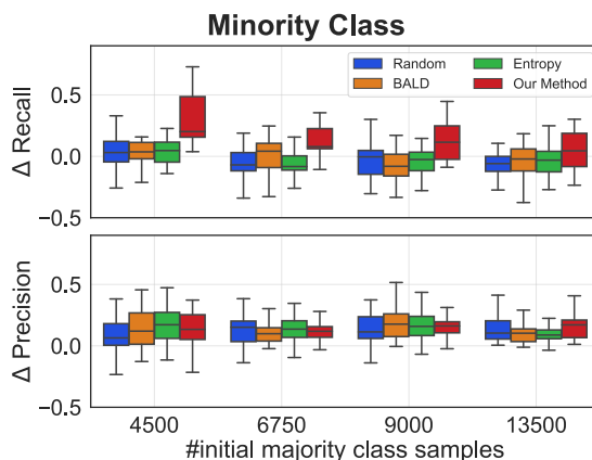
Fig. 5: Influence of initial AL training pool size: we report relative minority class performance gains for four dataset sizes with an increasing number of majority samples in the initial AL training pool. Performance differences are evaluated for each method, comparing model performance before the AL procedure with model performance after the procedure queried labels for 1000 samples. While performance gains of traditional AL methods decrease as the training dataset grows, our method retains more of the original performance increase.
