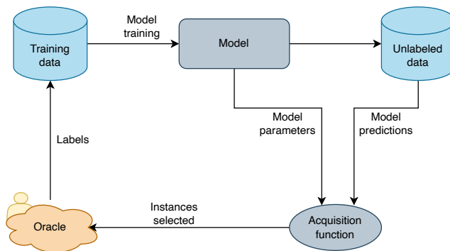
Fig. 1: Active Learning cycle: a model is trained on a pool of labeled data. Given the model predictions and parameters, an acquisition function selects informative samples from an unlabeled pool of data which are sent to the oracle for labeling.
