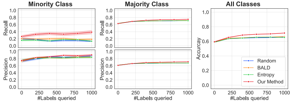
(a) CIFAR-10
