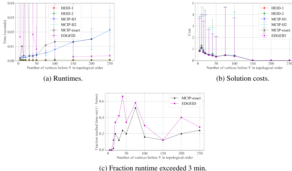
Figure 4: Experimental results for runtime, solution costs, fraction of graphs for which no solution was found, and fraction of graphs for which runtime limit of 3 minutes was exceeded. Error bars for runtime and cost graphs indicate 5th and 95th percentiles. Best viewed in color.
