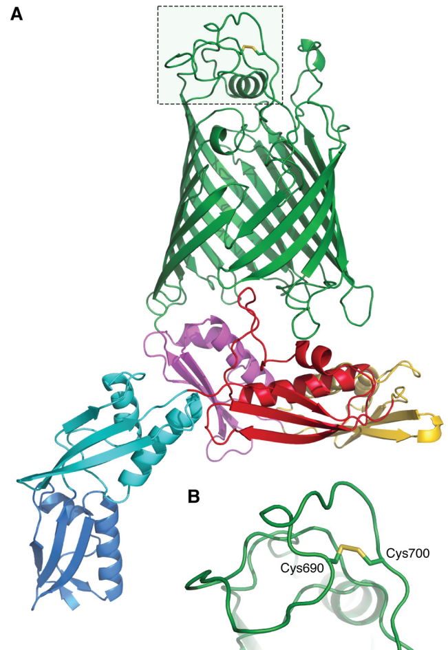
Figure 3. Structure of E. coli BamA. A , cartoon representation of E. coli BamA from PDB structure 5D0O (59). The transmembrane \beta -barrel domain of BamA is colored green and the five periplasmic domains POTRA1, POTRA2, POTRA3, POTRA4, and POTRA5 in blue, cyan, red, yellow, and magenta, respectively. B , the disulfide bond present in extracellular loop 6 of BamA (represented as sticks) is dispensable for folding and activity.
