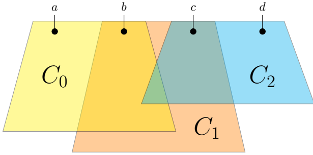
Fig. 1: Example of compatible and incompatible cuts
