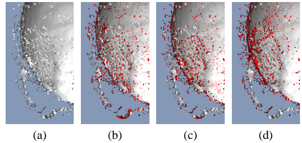
Figure 15: Three different outlier classifiers. Potential outliers marked in red. (a) Raw scanned geometry. (b) Classification using the miniball criterion. (c) Plane- t criterion. (d) k -nearest-neighbor graph criterion. All criteria were thresholded to classify 7% of the surfels as outliers.
