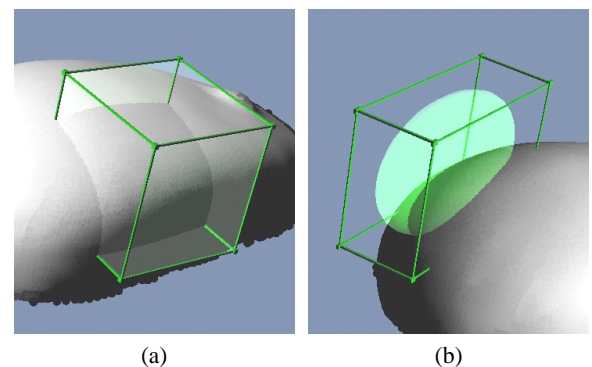
Figure 4: The volumetric brush. (a) A box shaped selector, following the object surface. (b) An ellipsoidal selector, freely positioned in space.
