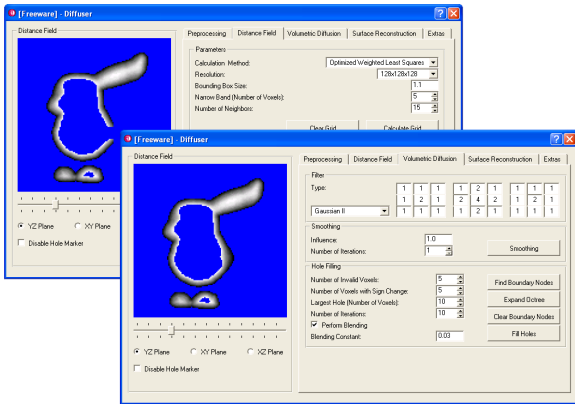
Figure 11: The user interface of the automatic hole filling tool allows to tune the algorithm. The volumetric representation can be previewed before surface reconstruction.
