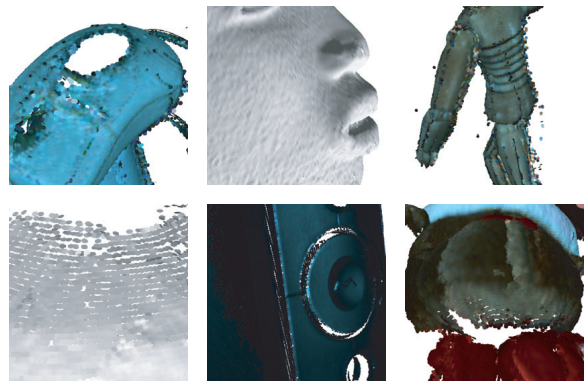
Figure 1: Typical artifacts of raw scanner data. Top Row: Holes due to sensor restrictions, noise, outliers. Bottom Row: Low sampling density due to gracing sensor views, low sampling density at delicate surface details, and holes due to critical reflectance properties.
