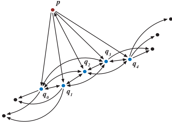
Figure 8: Nearest-neighbor graph. Depicted are the 5-nearest-neighbor relations for p and its 5-neighbors q_0, \dots, q_4 . Note that only q_2 shares a reciprocal neighbor relationship with p .
