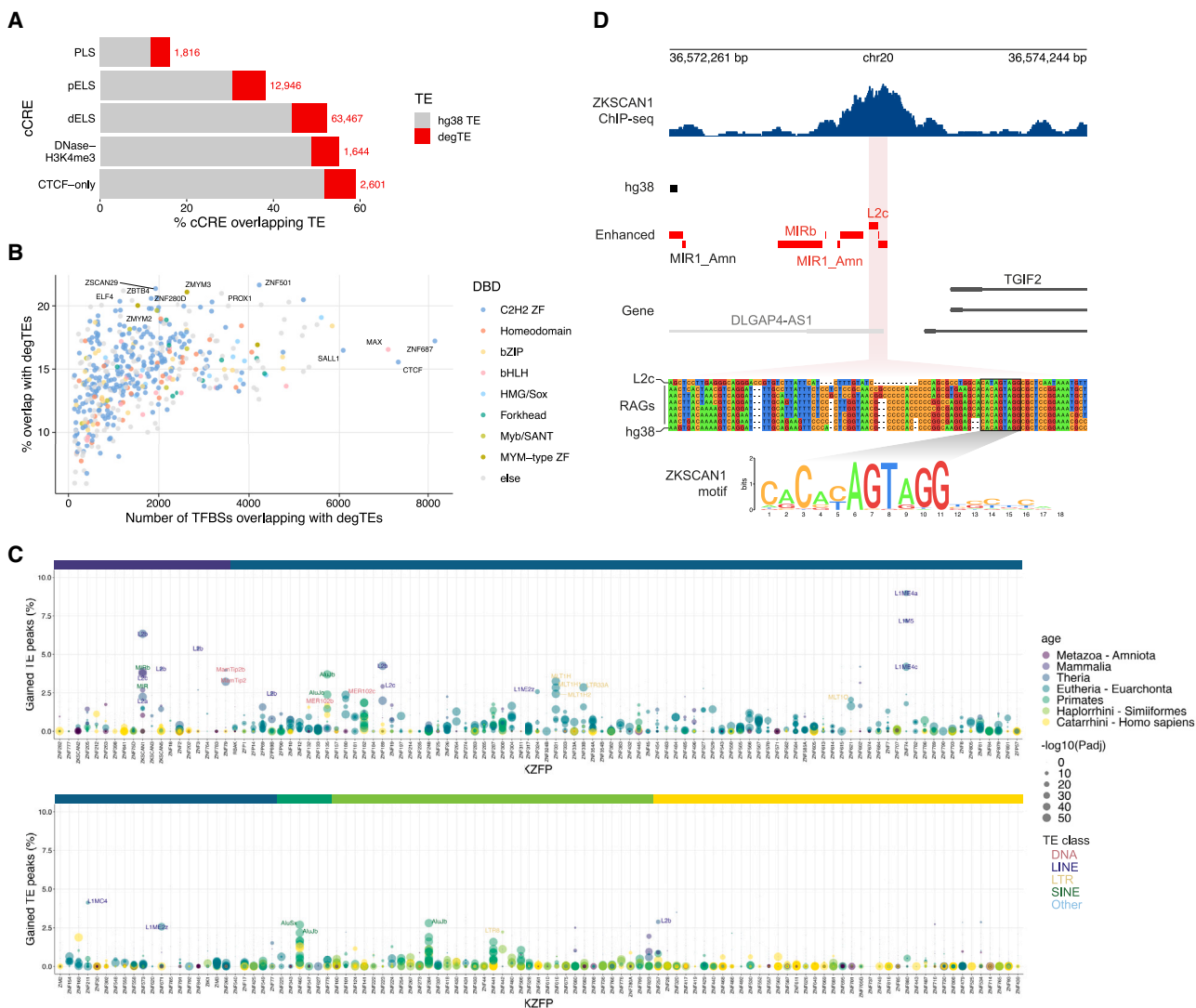
Figure 4. cCREs and TFBSs derived from degTEs
