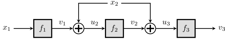
Fig. 2: The TNT construction by Bao et al. [2].
