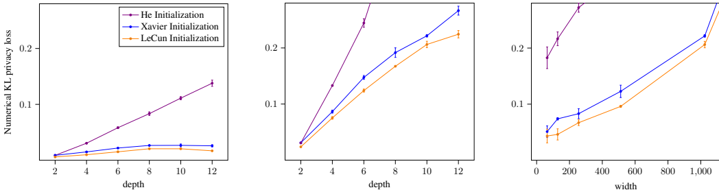
(a) Privacy vs depth (20 epochs, \sigma = 0.01 , width = 1024)
