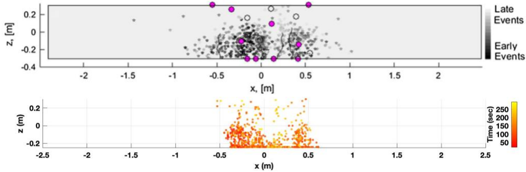
Figure 2. Sample comparison between 380 AE sources localized by manual processing [top, Figure from [7]] and 1038 AE sources using SIMORGH (bottom) for the flexural beam loaded to 111 kN (25 kip). Purple circles show the sensor locations. Curved lines show the observed cracks at the end of the experiment.
